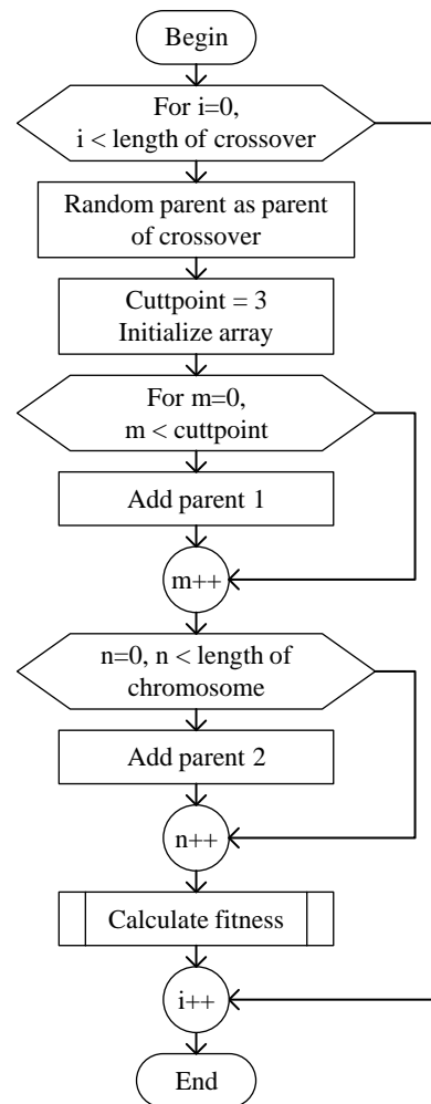
Fig. 3. Flowchart of crossover process
